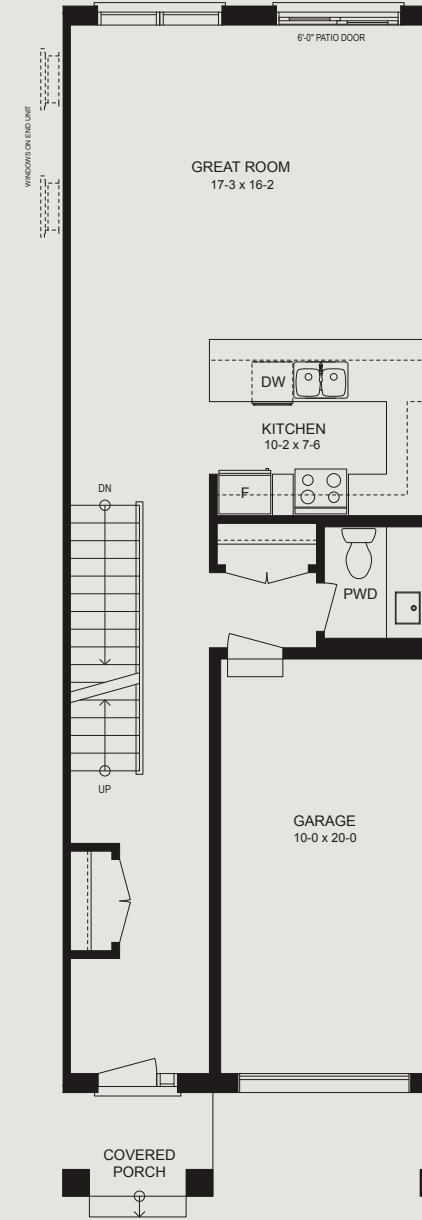
INTERIOR UNIT MAIN FLOOR
